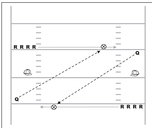
Figure 2-16. Pat-and-go drill
